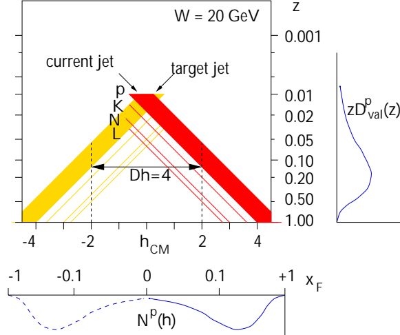
FIGURE 5. Relation between z -values in fragmentation and CM rapidity for W = 20 GeV. Roughly speaking, for regions separated by at least four units in CM rapidity, current and target fragmentation can be kinematically separated.
