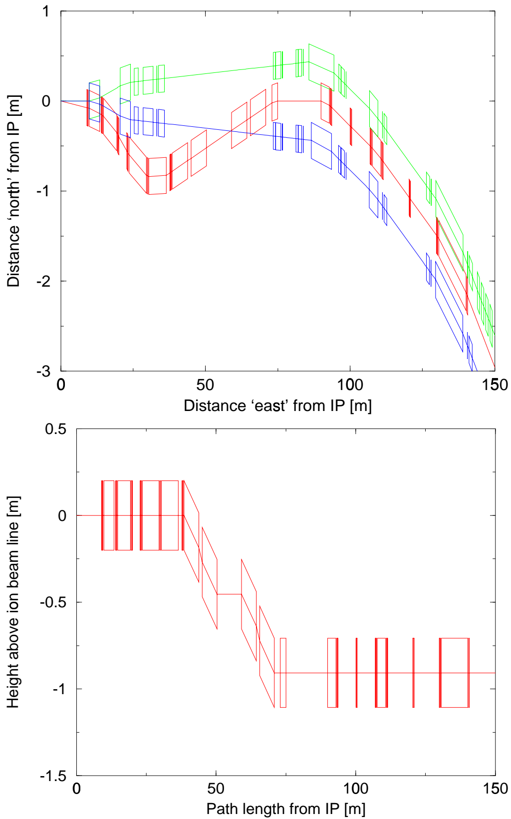
Fig. 7. Plan and side views of the eRHIC magnet layout in an interaction region WITHOUT spin rotators.
