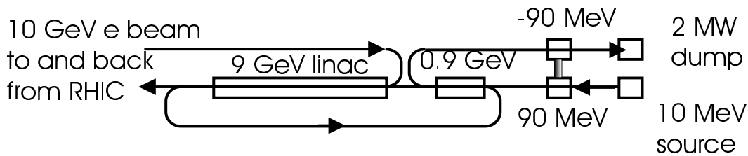
Fig. 3. Schematic layout of a two stage recirculating linac structure in the linac-ring collision scenario.
