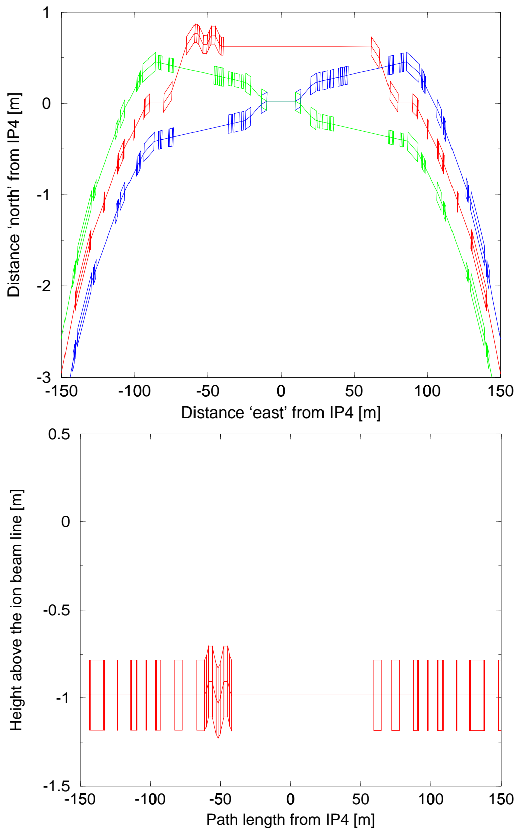
Fig. 10. Plan and side views of the magnetic layout around the utility region IP4, including a Siberian snake of the first kind.
