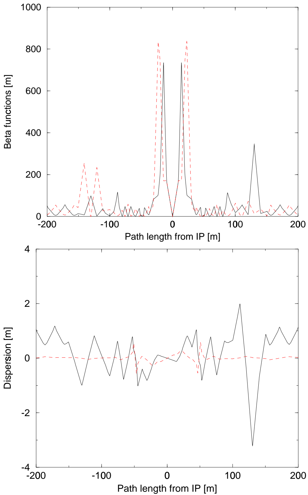
Fig. 9. Beta and dispersion functions around an IP with spin rotators.
