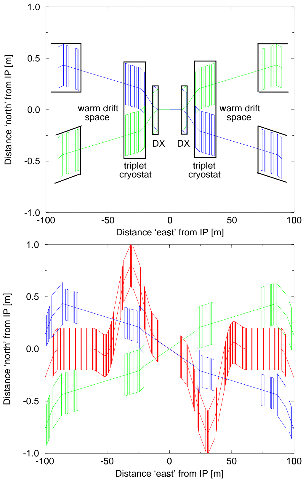
Fig. 6. The magnet layout close to the IP in nominal RHIC operation during gold-gold or proton-proton collisions (top), and after modification for eRHIC (bottom).
