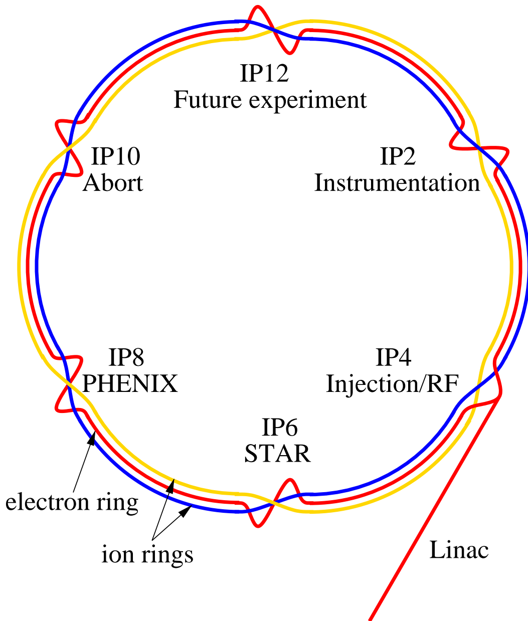
Fig. 1. Schematic layout of the injection linac, electron ring, and the two ion rings, in the ring-ring collision scenario.
