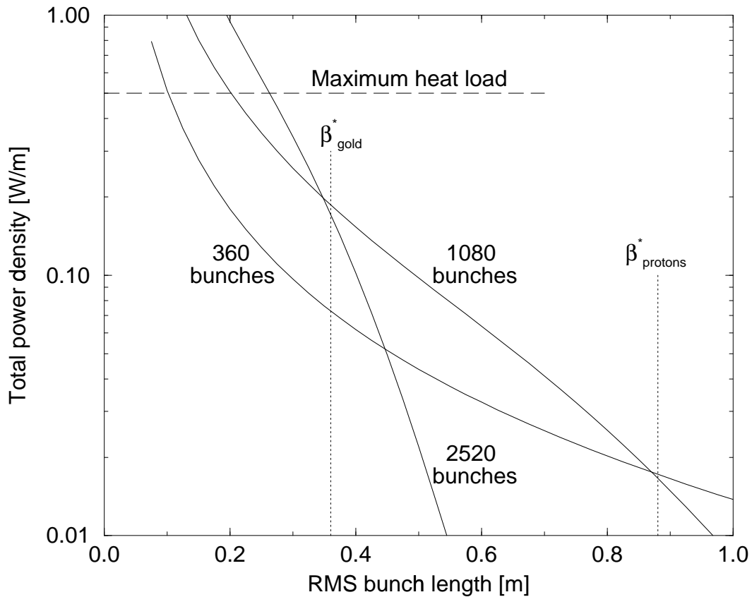
Fig. 11. Linear power load deposited at cryogenic temperatures in the stainless steel vacuum chamber of the ion rings, due to beam image currents, for a total charge of 0.93 \times 10^{11} per bunch – at the beam-beam limit for the electrons.
