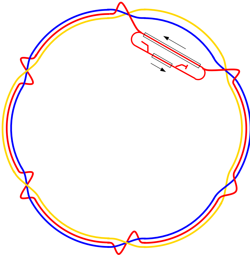
Fig. 4. Schematic layout for linac-ring collisions, using the RHIC tunnel to return the 10 GeV electrons for energy recovery.
