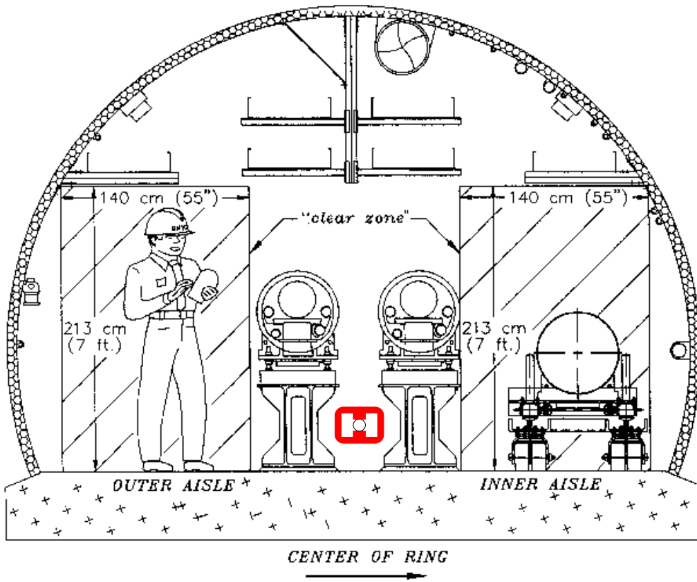
Fig. 2. RHIC tunnel cross-section, showing an electron ring magnet between the ion ring stands.
