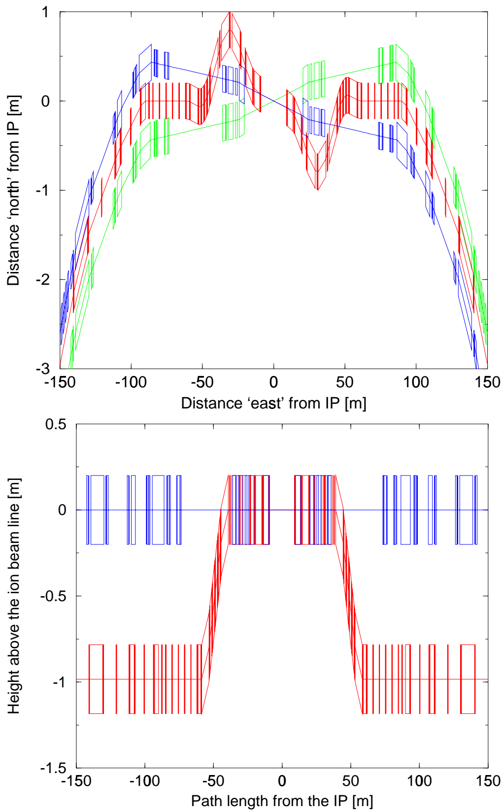
Fig. 8. Plan and side views of the eRHIC magnet layout in an interaction region WITH spin rotators.
