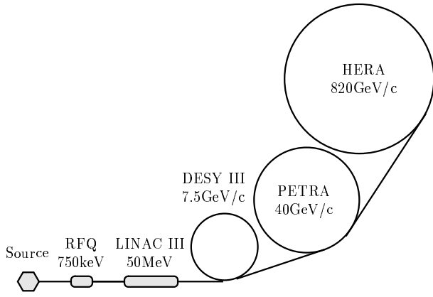
Figure 5: The accelerator chain at DESY for high energy collisions in HERA.
